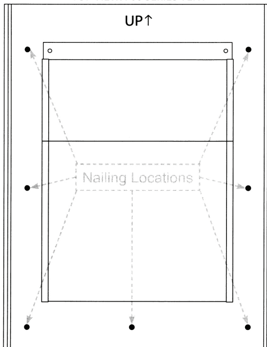
TOP VIEW: 700 SERIES VENT
